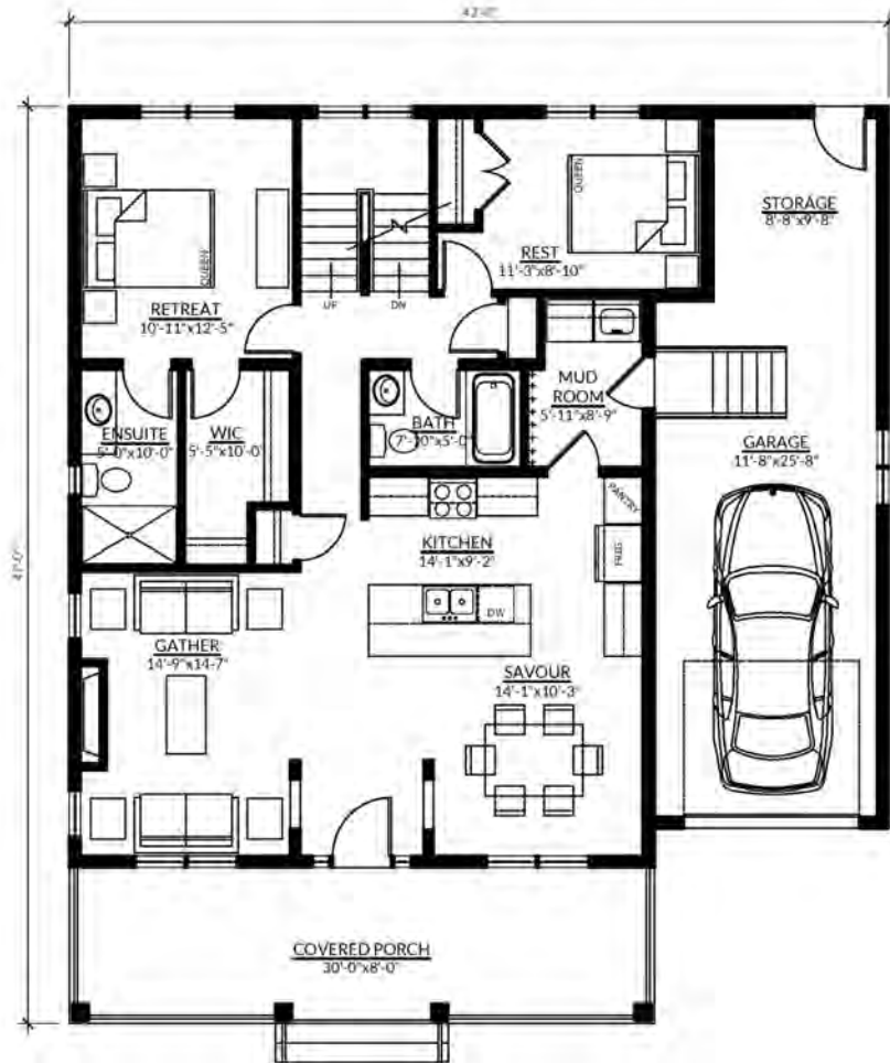
MAIN FLOOR - 1200 sq ft
