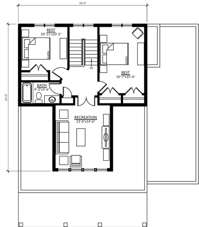
LOFT - 780 sq ft
